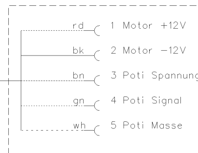
Aktuator links
